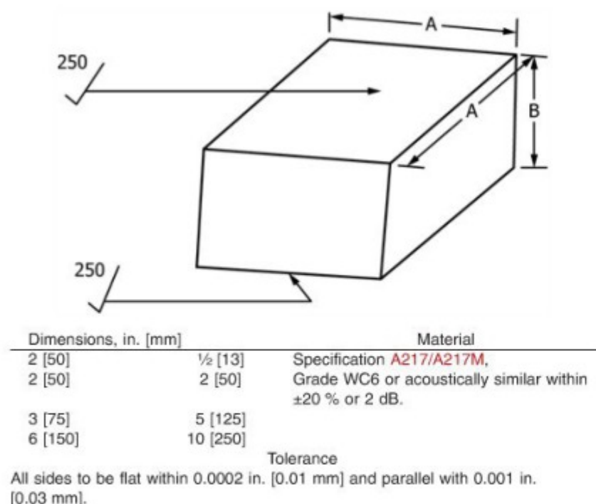
FIG. 3 Calibration Blocks
